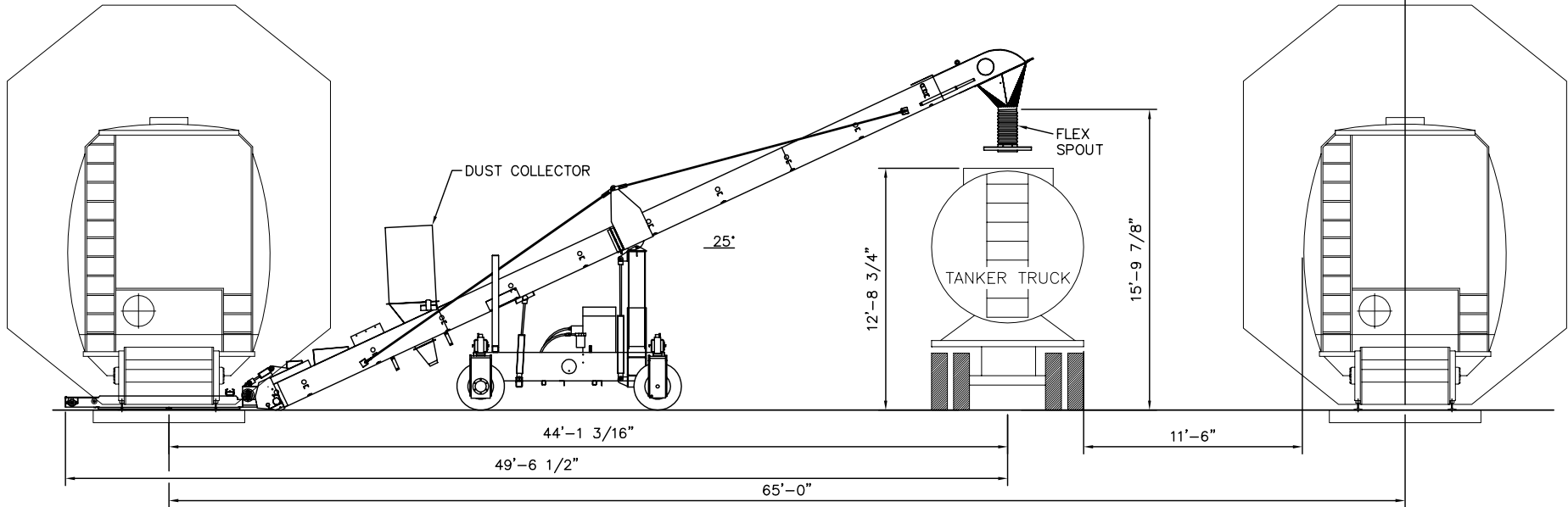
MODEL #1850, MODEL #2450
